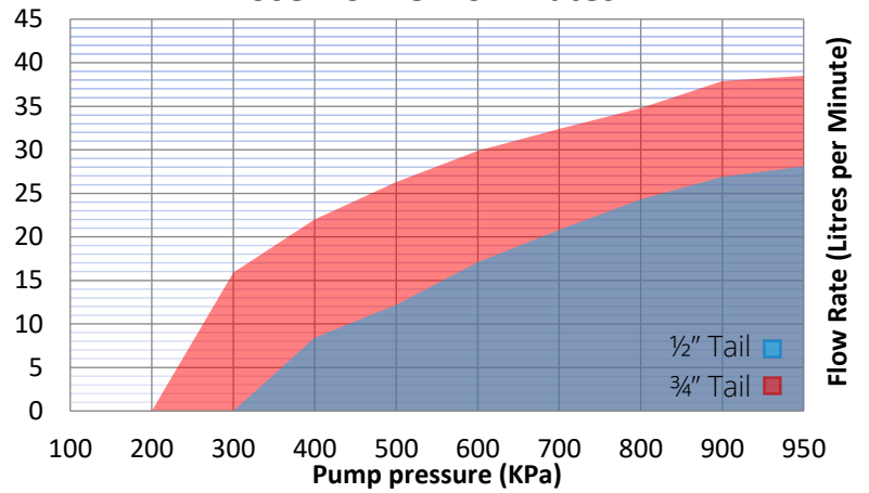
102-A-NZL10045 Low Flow Hose Nozzle to 1" FBSP
